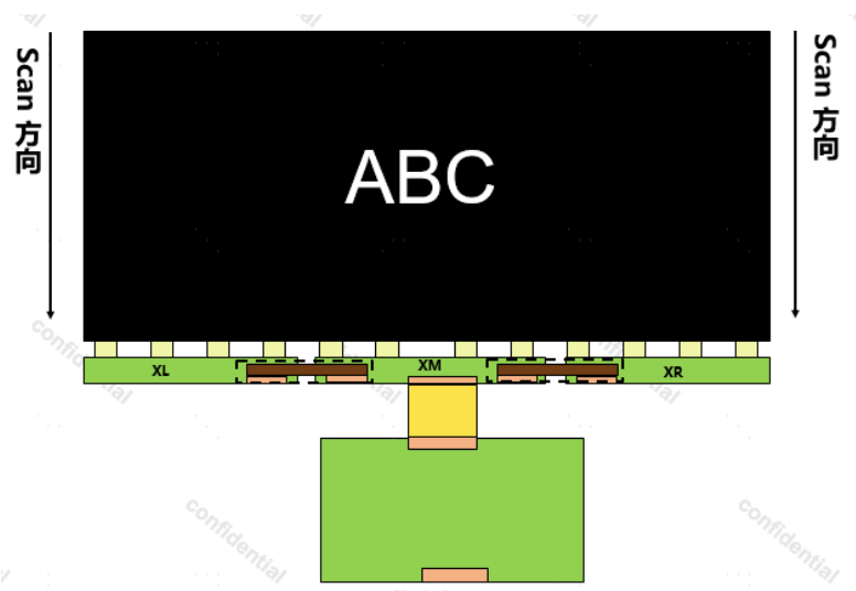
Fig 1.1 Display Orientation
