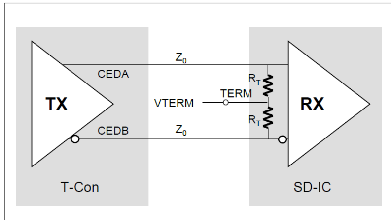
Fig. 3.2 Internal Termination Resistor
