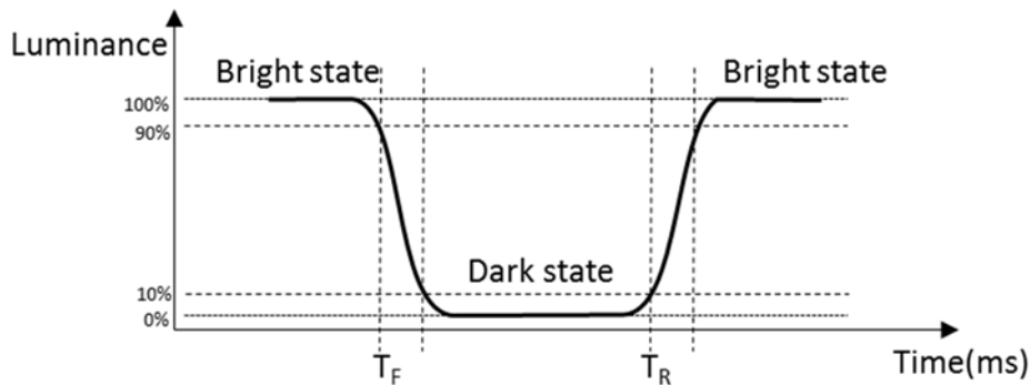
Fig. 4.4 The Definition of T_R and T_F
