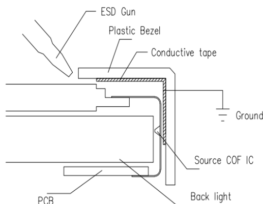
Fig. 3.7 Source COF IC ESD Protection
