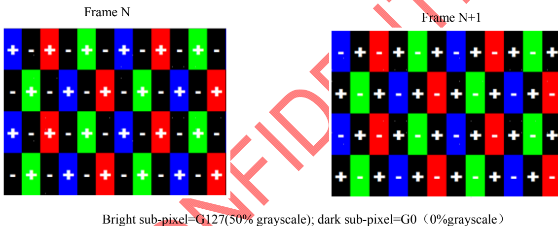
Fig 3.6 Flicker Pattern
